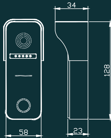
DOORBELL (OUTDOOR UNIT)
